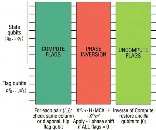
Figure 3. Structure: Compute → Phase Flip → Uncompute.
