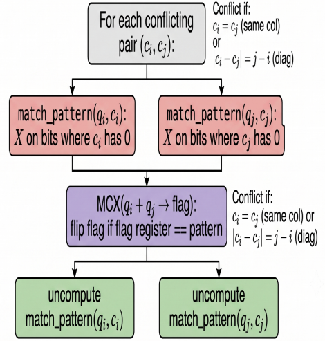
Figure 4. Conflict detection (c_i, c_j) with match_pattern .
