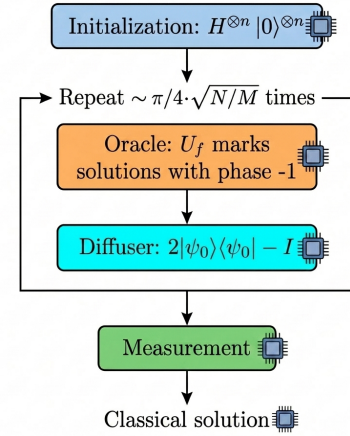
Figure 1. Flow of Grover's algorithm for N-Queens.
