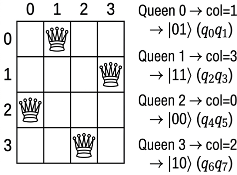
Figure 2. Encoding of [1,3,0,2] for N = 4 : 2 qubits per queen.
